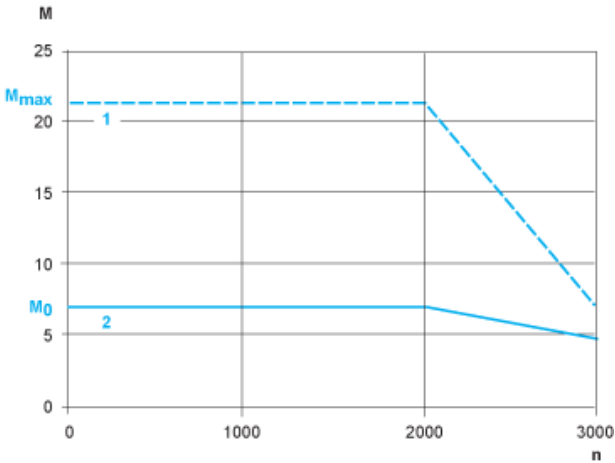
Servo Motor with LXM23•U15M3X Servo Drive
