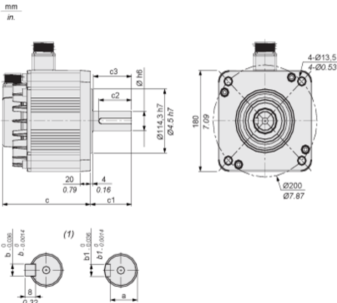
(1) Shaft end, keyed slot (optional) Dimensions in mm
