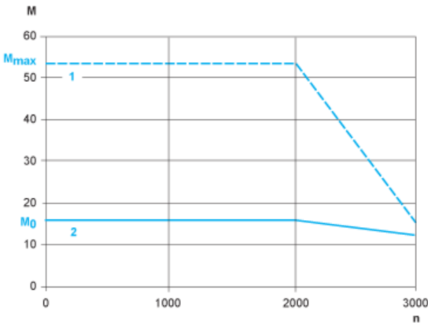
Servo Motor with LXM23•U30M3X Servo Drive
