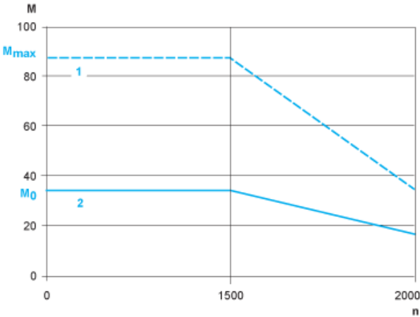
Servo Motor with LXM23•U55M3X Servo Drive
