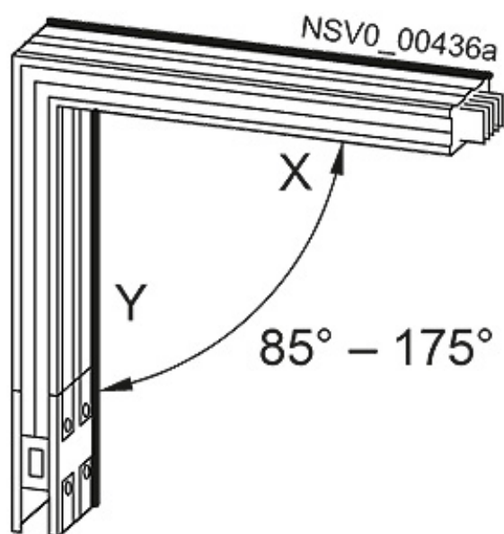
BD2A-400-LH-X*/Y*-G* KNEE BACKSIDE X/Y 0,36M-1,25M 1 60A-400A WINKEL 85 GRAD-175 GRA D
