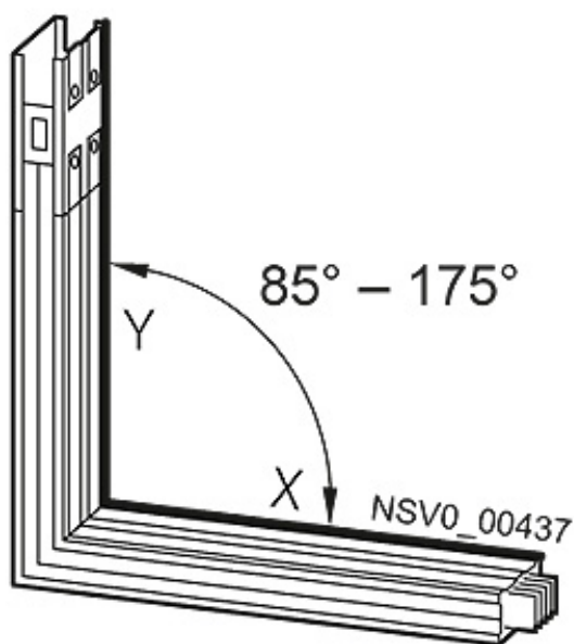
BD2C-1250-LV-X*-G* KNEE FRONTSIDE X 0,36M-1,25M / Y 0,36M 1250A WINKEL 85 GRAD-17 5 GRAD
