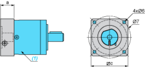
(1) Gearbox Values in mm
