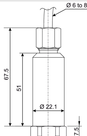
Housing with cable outlet, 3-wire, 1.5 m length
