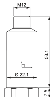
Housing with connector M12-A, 4-pin
