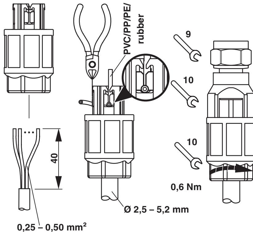
Functional drawing
