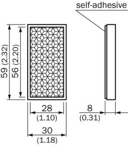
All dimensions in mm (inch)
