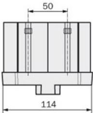
Sliding nut groove for side mounting
