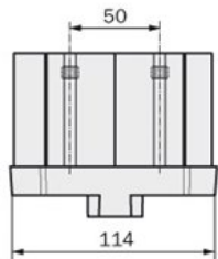
Sliding nut groove for side mounting
