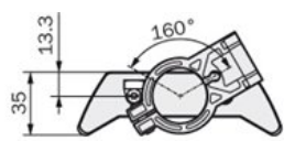
Mounting with swivel mount bracket (Part No. 2019659)
