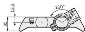
Mounting with swivel mount bracket (Part No. 2019659)
