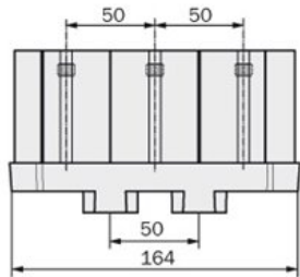
Sliding nut groove for side mounting
