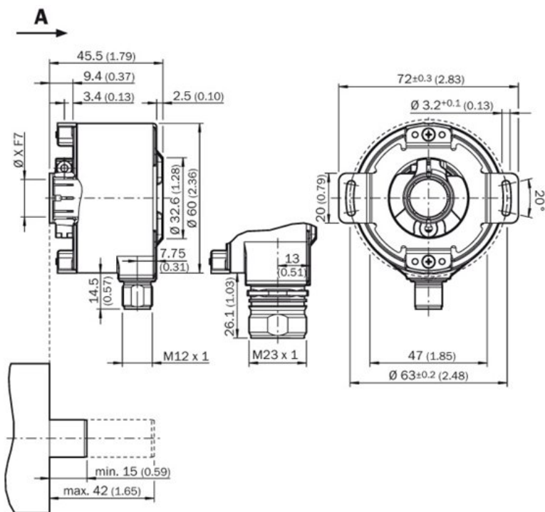
View of M12 device connector on encoder
