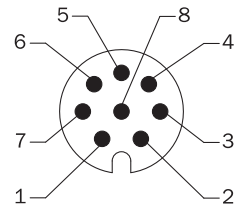
View of M12 male device connector on encoder
