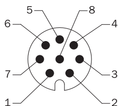
PIN Wire colors (cable connection) Signal Explanation 1 Brown Data - Interface signals 2 White Data + Interface signals 3 Black V/R Sequence in direction of rotation 4 Pink SET 5 Yellow Clock + Electronic adjustment Interface signals 6 Purple Clock - Interface signals 7 Blue GND Ground connection 8 Red U S Operating voltage Screen Screen connected to housing on encoder side. Connected to ground on control side.
