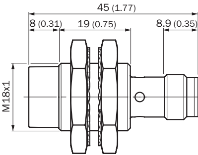
IMB18 Short-body housing, connector M12, non-flush
