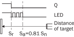
Installation aid
