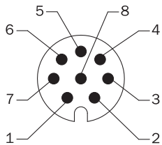
PIN Wire colors (cable connection) Signal Explanation 1 Brown Data - Interface signals 2 White Data + Interface signals 3 Black V/R Sequence in direction of rotation 4 Pink SET Electronic adjustment Interface signals 5 Yellow Clock + Interface signals 6 Purple Clock - Interface signals 7 Blue GND Ground connection 8 Red U S Operating voltage Screen Screen connected to housing on encoder side. Connected to ground on control side.
