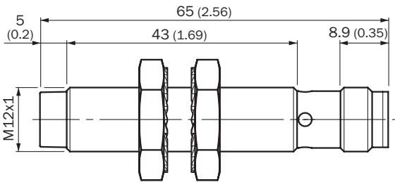
IMB12 Standard, connector M12, non-flush
