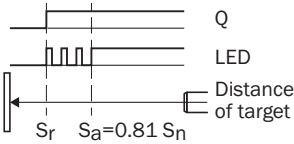
Installation aid
