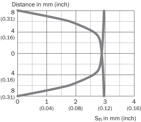
Response diagram
