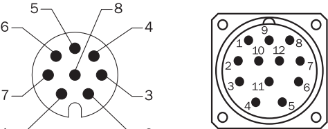
View of M12 / M23 male device connector on cable / housing
