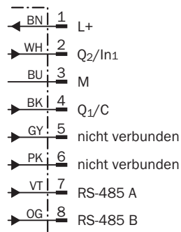
SPS RS-485, IO-Link (Q) 1 x I/O
