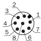
SPS RS-485, IO-Link (Q) 1 x I/O
