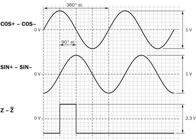
For clockwise shaft rotation, looking in direction “A” (see dimensional drawing) Signal SIN/COS before differential generation
