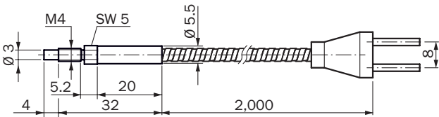
Dimensional drawing (Dimensions in mm (inch))
