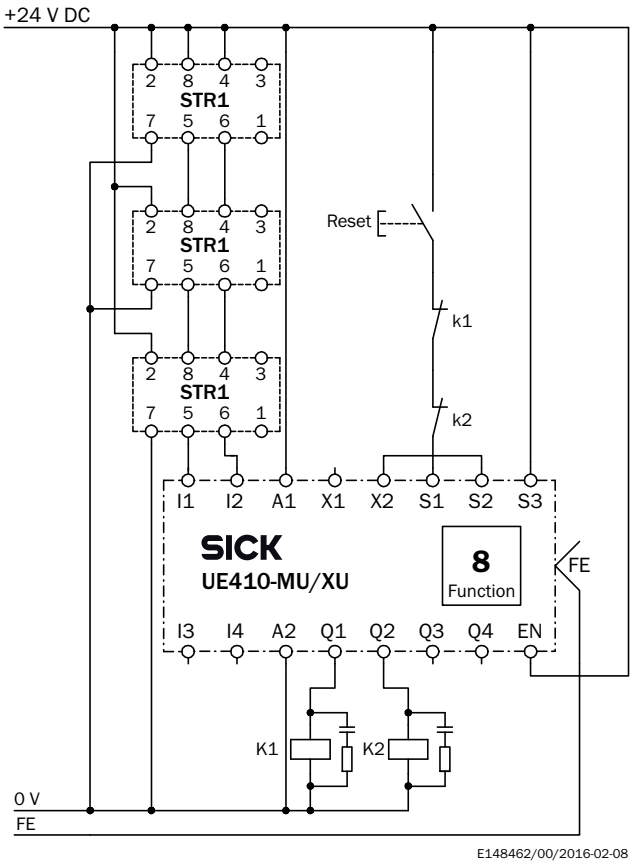
Series connection of three STR1 transponder safety switches to a Flexi Classic safety controller
