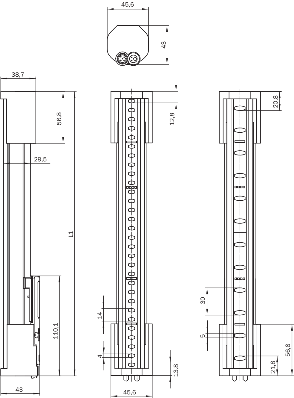
Dimensional drawing (Dimensions in mm (inch))
