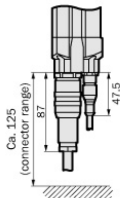
Cable socket M26 with crimp contacts (for DIN 43 651, left) and cable plug M12 with cable (right, only on receiver)
