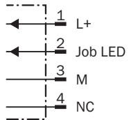
Sender
