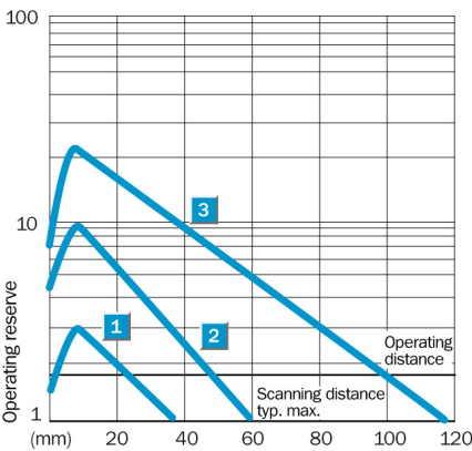
Characteristic curve
