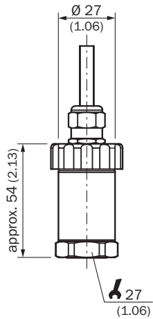
Housing with flying leads
