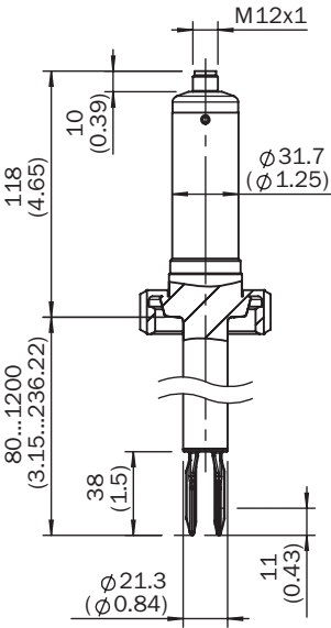
Dimensional drawing
