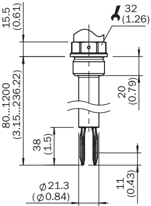
Dimensional drawing housing
