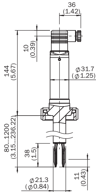
Dimensional drawing
