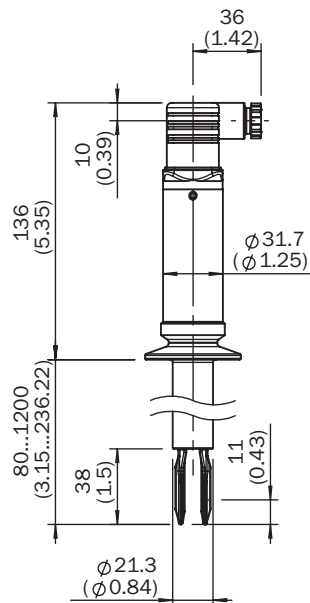
Dimensional drawing
