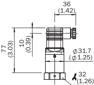
Dimensional drawing housing
