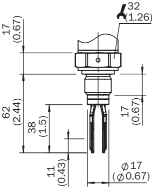
Dimensional drawing housing
