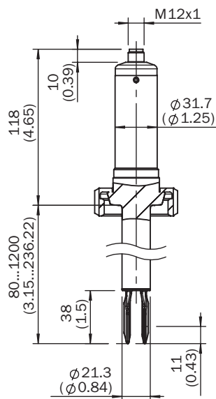
Dimensional drawing
