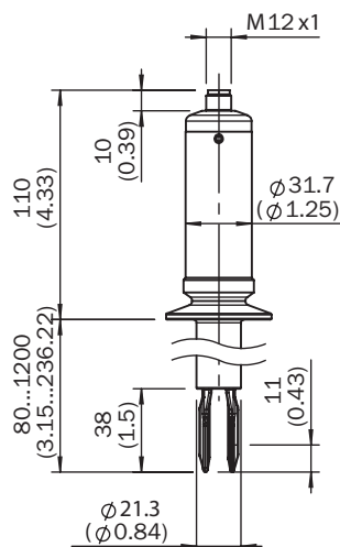
Dimensional drawing
