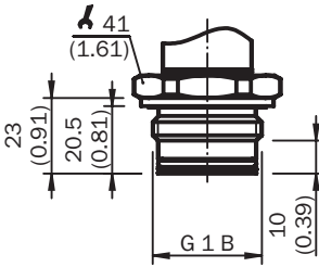
G 1 B with cooling section
