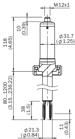
Dimensional drawing
