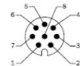
View of M12 device connector on encoder
