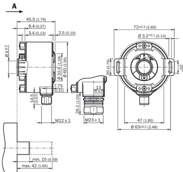
View of M23 device connector on encoder
