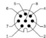
View of M12 device connector on encoder
