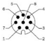
View of M12 device connector on encoder
