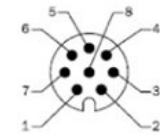
View of M12 device connector on encoder
