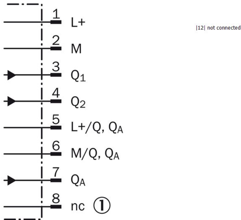
Connection diagram DMxxx-2 RS232/RS-422, PG9
