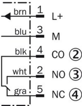
Receiver
