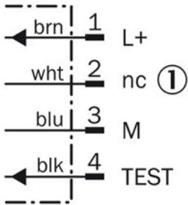
Sender
