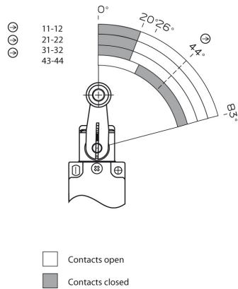
Actuator travel diagram
