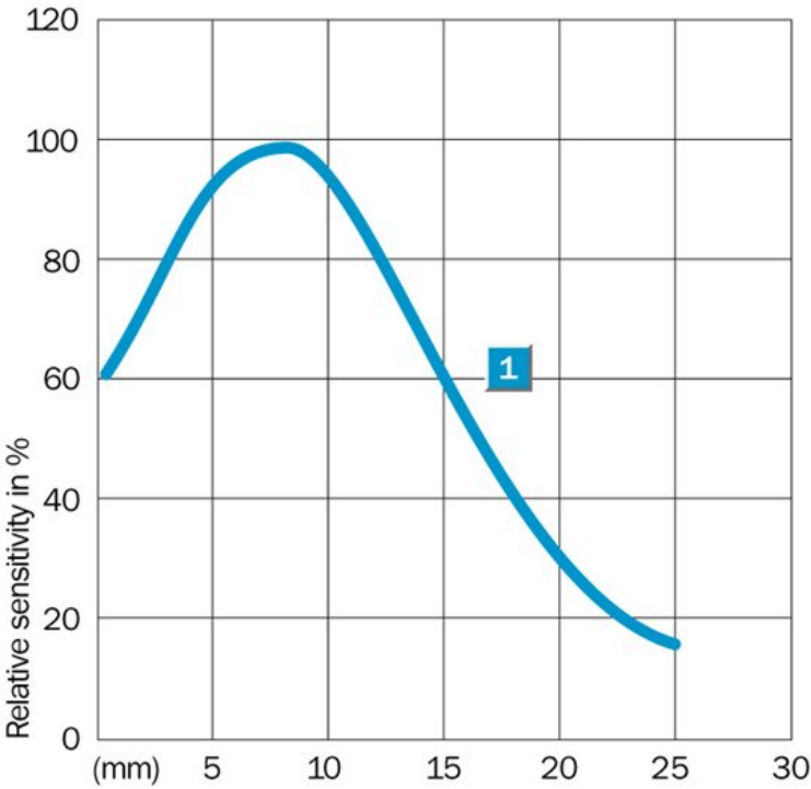
Characteristic curve
