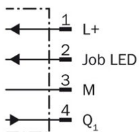
Receiver
